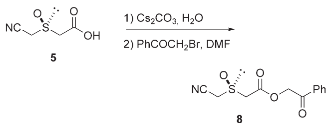
Figure 4. Preparation of benzoylmethyl cyanomethylsulfinylacetate ( 8 ).
