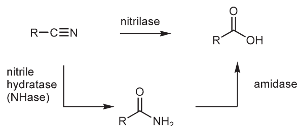
Figure 1. Nitrile hydrolysing enzymes.
