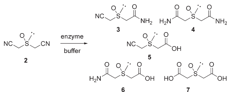
Figure 3. Possible products of hydrolysis of ( 2 ).
