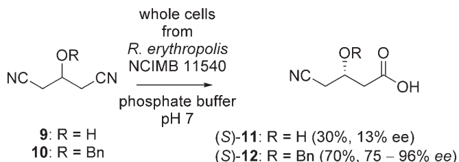
Figure 5. Hydrolysis of hydroxyglutaronitriles.
