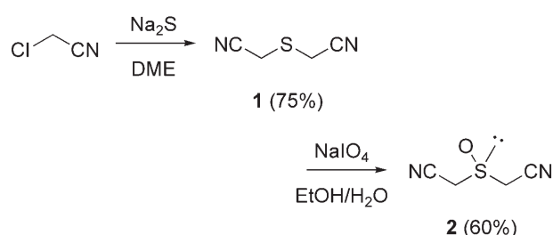
Figure 2. Synthesis of bis(cyanomethyl) sulfoxide ( 2 ).
